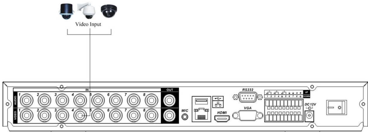
Figure 3-1 1U
