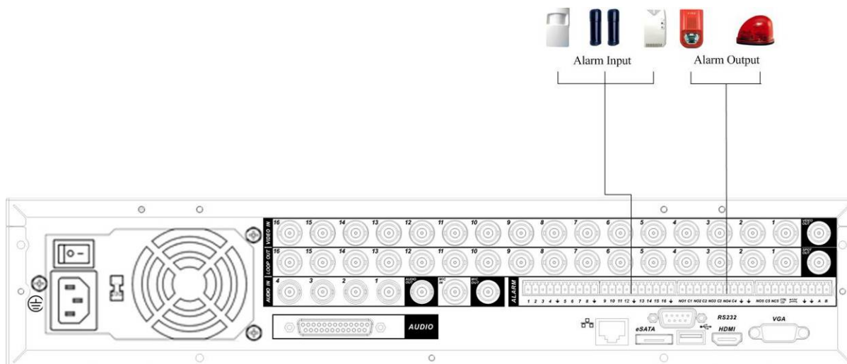
Figure 3-15 2U
