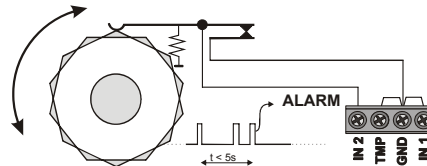
Ratchet-wheel function scheme
