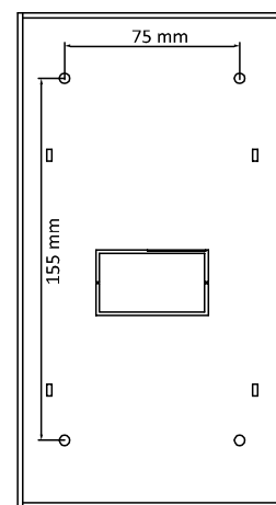
Rear View
