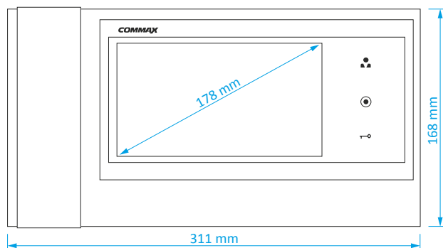
CDV-70K / CDV-70KR3
