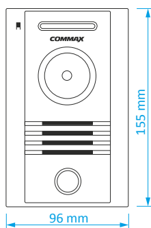
DRC-40K
