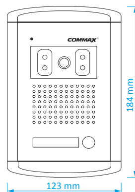
DRC-4CAN
