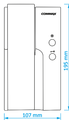
DP-4VHP / DP-2HPR
