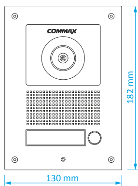
DRC-41UN
