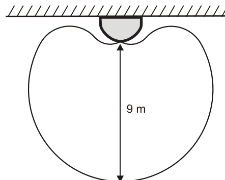
Detector relative directional sensitivity
