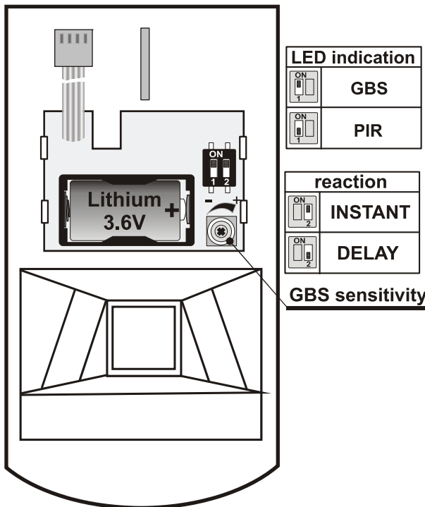
Glass-break detector
