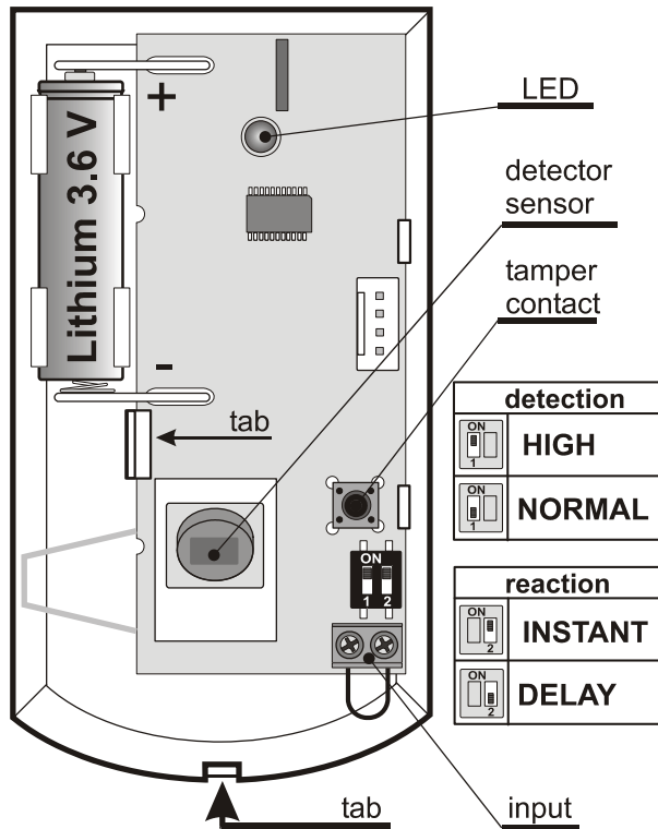
PIR movement detector
