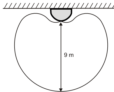
Glass-break detector relative directional sensitivity
